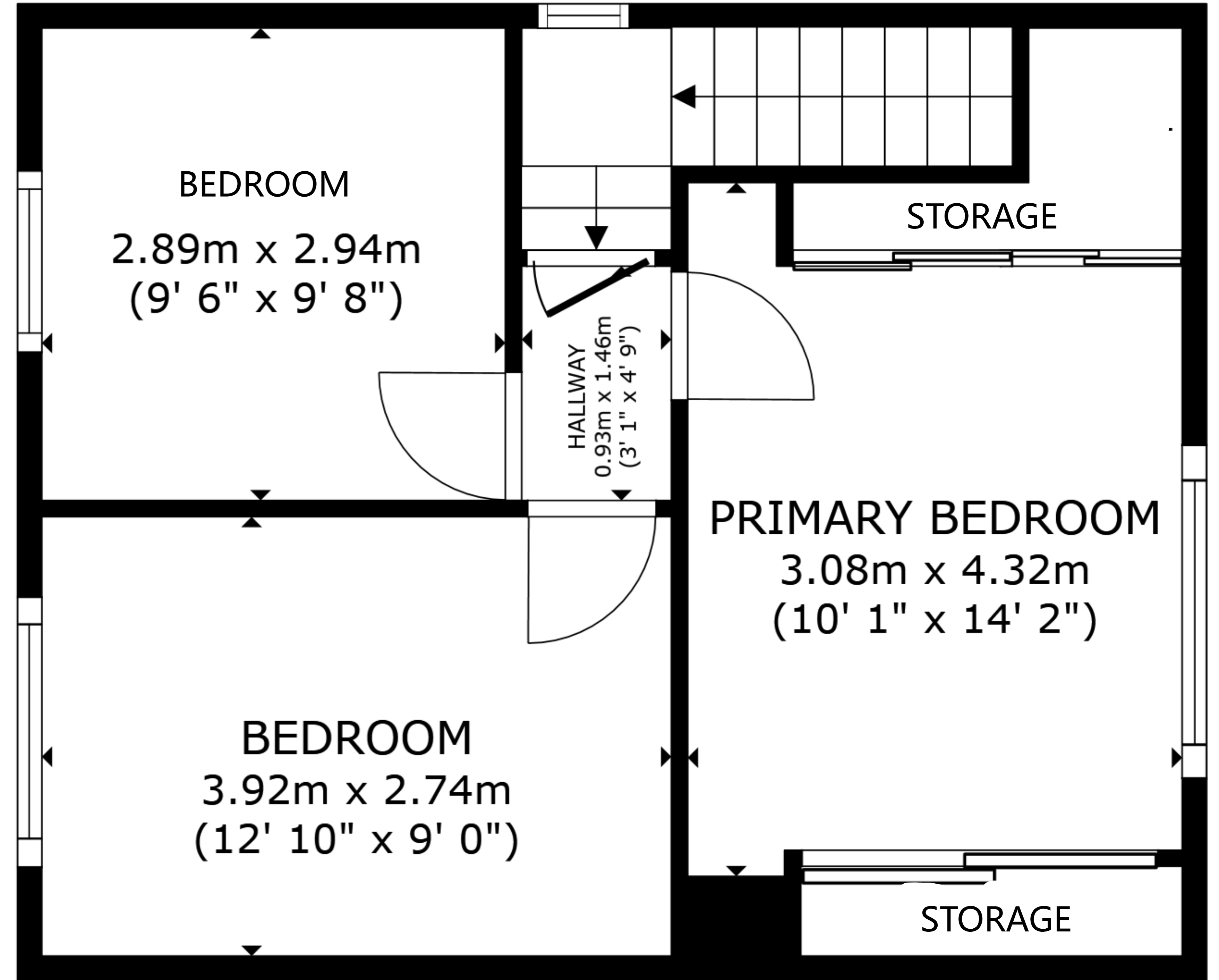
FLOOR 2
