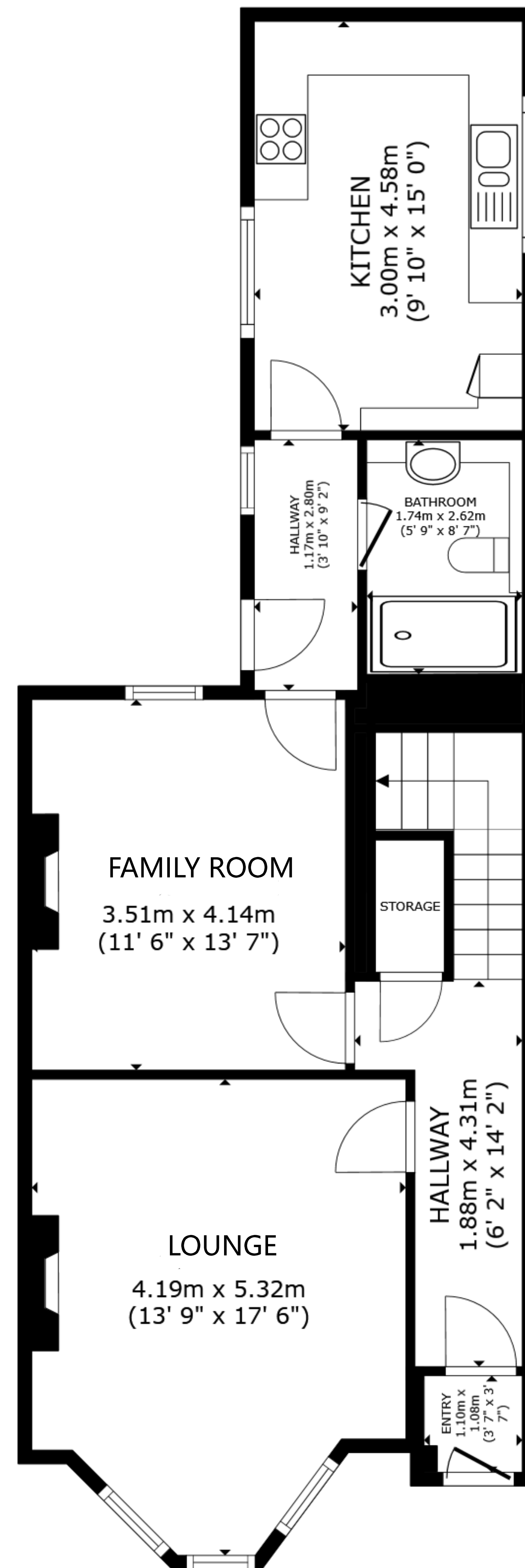
FLOOR 1
